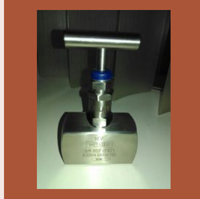
SS High Pressure Needle Valve
